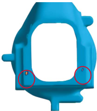
Porosity in a ductile iron housing
