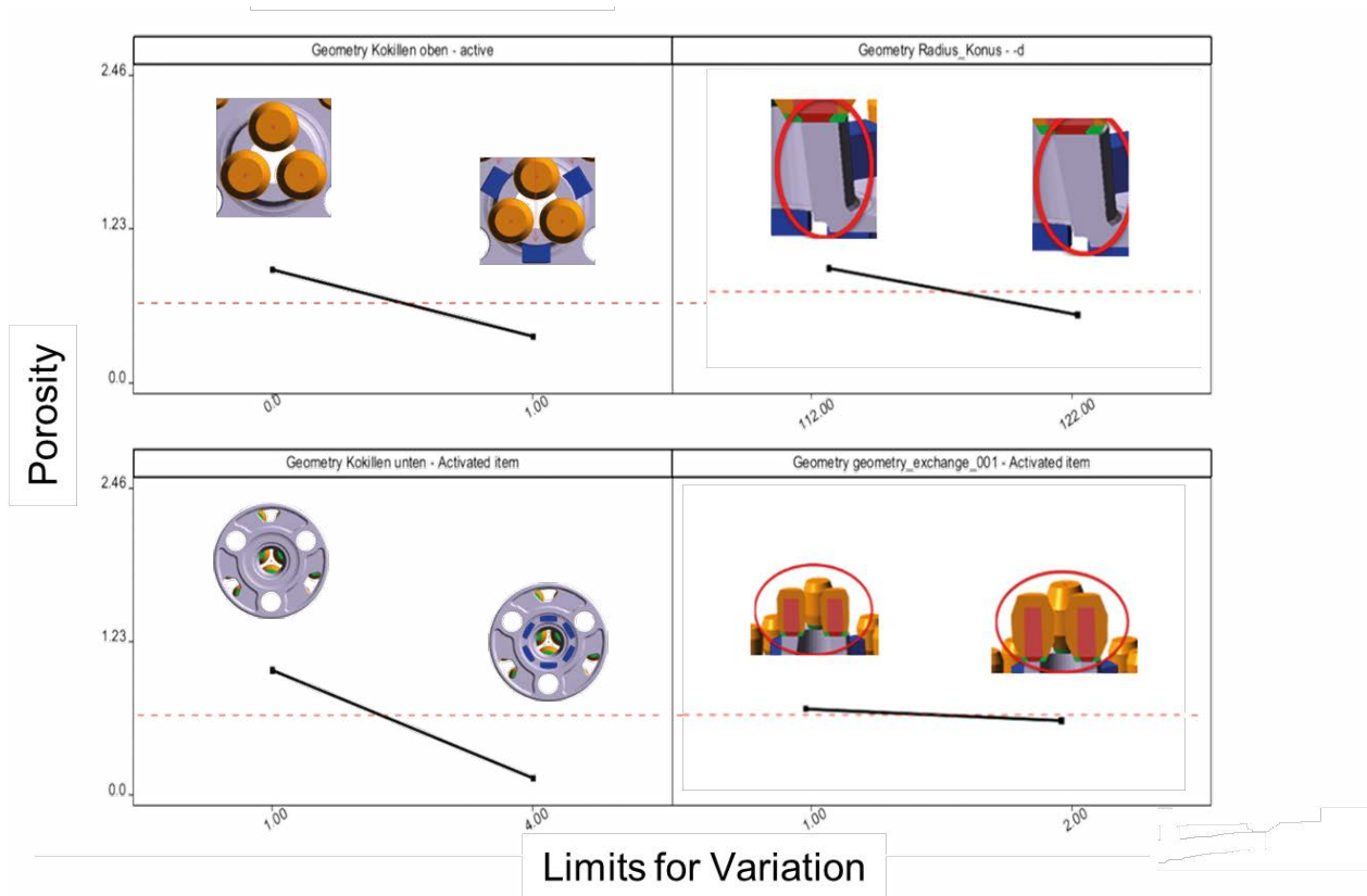
Quantitative determination of main influencing variables on porosity in a casting (feeder sizes, chills, padding)
